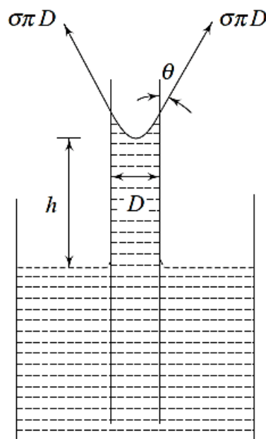
Capillary rise
