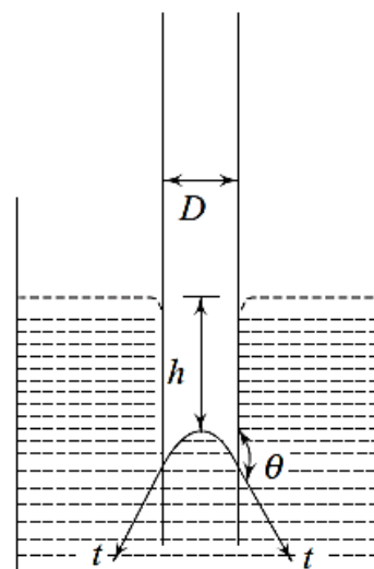
Capillary depression
