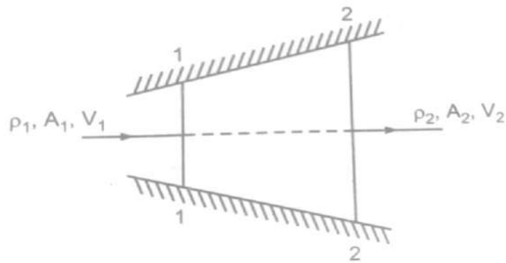
FIG. 5.13 Fluid flowing in a pipe
