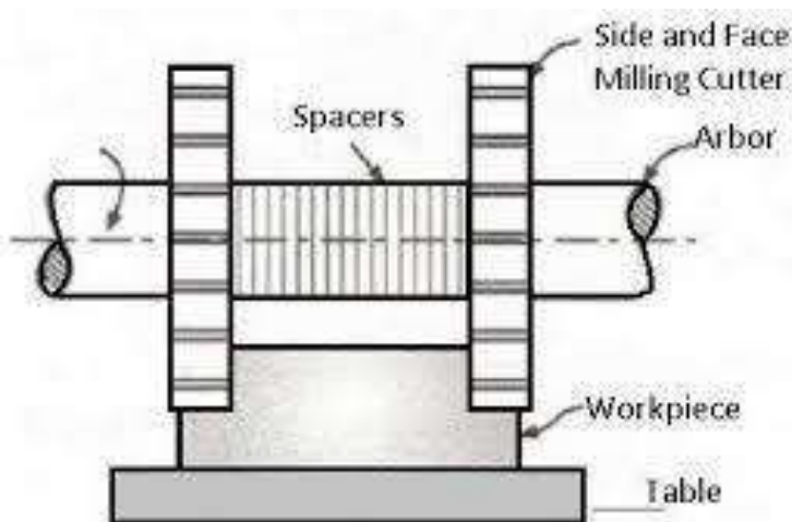
Straddle Milling Operation
