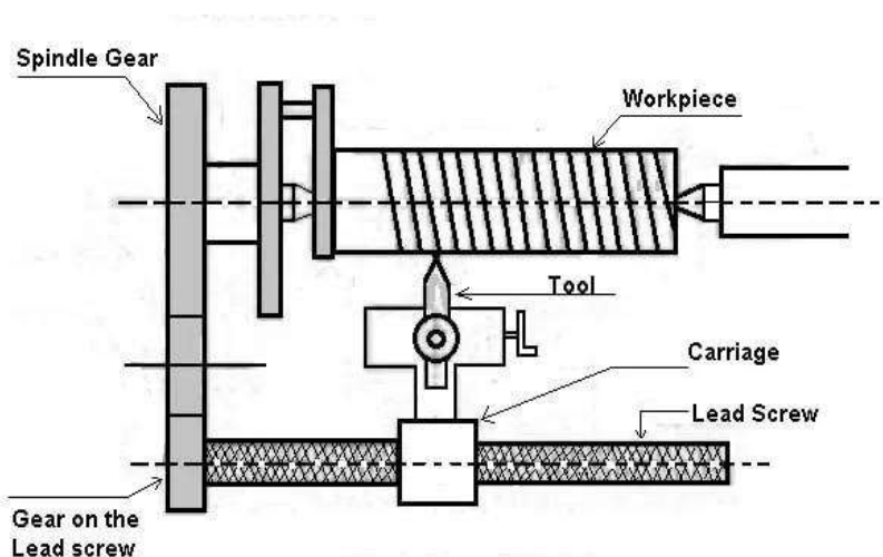
Thread Cutting
