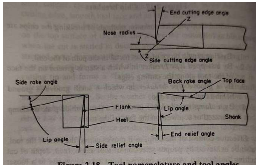
Figure 2.18 Tool nomenclature and tool angles
